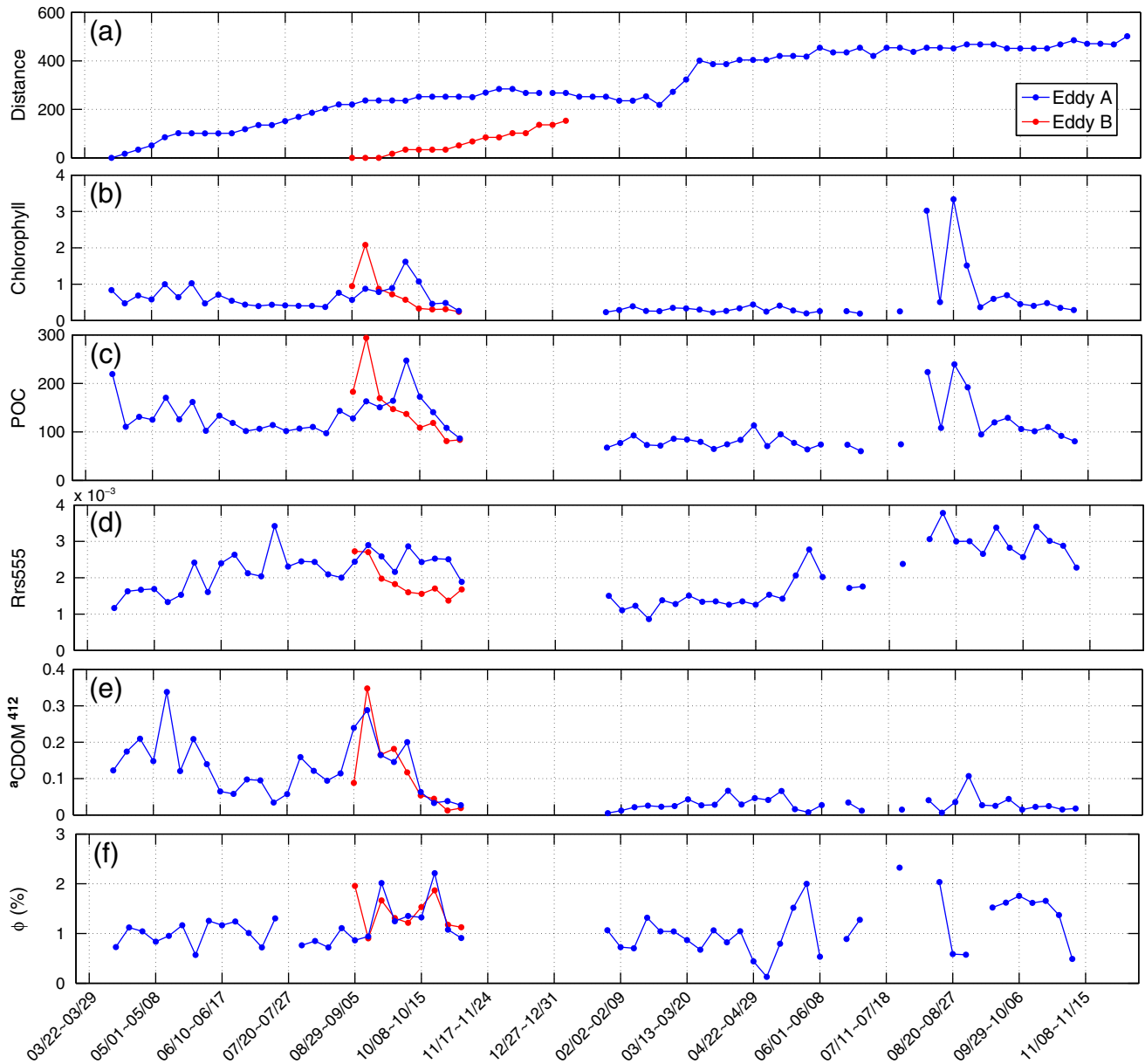
Fig. 3. Lagrangian views of the temporal evolution of satellite-derived characteristics of the target eddy during 2011–2012. Distance (a, km) is calculated between eddy center and its starting location near Haida Gwaii from altimeter data. Time series of MODIS/Aqua derived surface chlorophyll (b, mg m -3 ), POC (c, mg C m -3 ), surface turbidity as Rrs555 (d, Sr -1 ), aCDOM412 (e, m -1 ), and quantum yield of fluorescence φ (f, relative) averaged within the eddy core from 8-day composites for eddy A (blue line), and eddy B (red line). (For interpretation of the references to color in this figure legend, the reader is referred to the web version of this article.)
